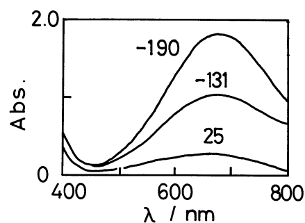
Fig. 5. Temperature dependence of a CT band that appeared in the CA/MDA system. Numerical values in the figure denote measurement temperatures in ^{\circ}\text{C} .
